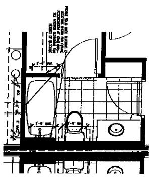
Typical Bathroom Blocking Plan-1st Floor Only
